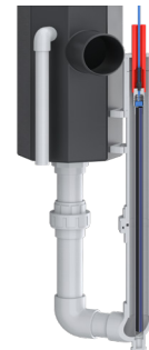
The Batchpur UV-module is connected behind the sampling container.
